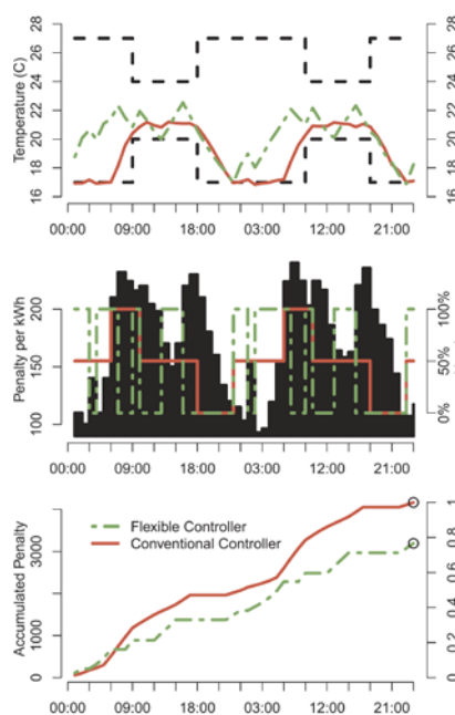
Top plot: An example of the temperature in a building controlled by a penalty-aware controller (green, dashed) and a conventional controller (red, solid). Both controllers are restricted to stay within the dashed lines.
