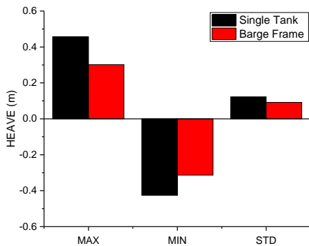
Figure 12. Heave motion statistical results for cases of single tank and tank enclosed by barge frame.
