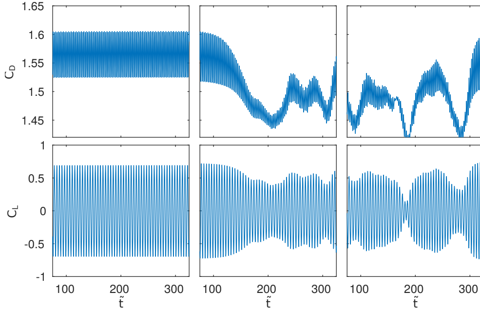
Figure 4. The computed instantaneous drag and lift coefficients, C_D and C_L respectively, for Reynolds numbers 180 (left), 190 (middle) and 210 (right) as a function of the dimensionless time \tilde{t} = t\bar{U}/D .
