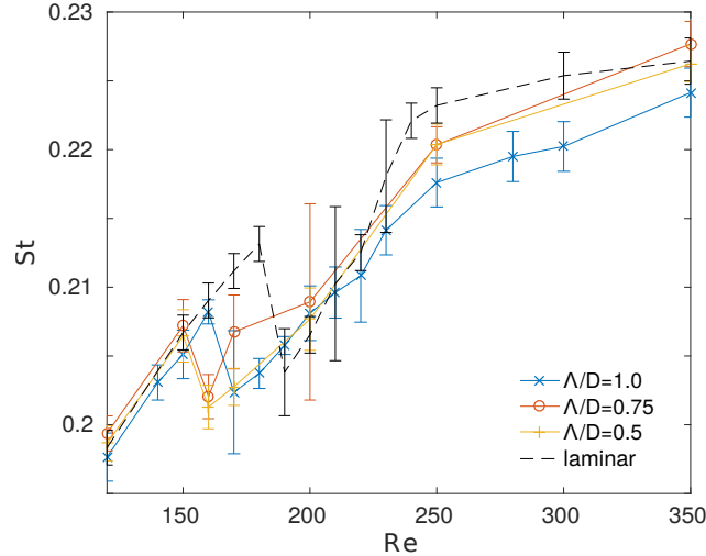
Figure 12. Comparison of St-Re relationships for flows with TFS with T_i = 25\% and different integral scales: -x- \Lambda/D = 1.0 ; -o- \Lambda/D = 0.75 ; -+- \Lambda/D = 0.5 ; - - LFS.
