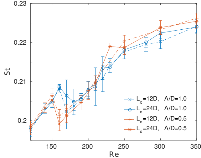
Figure 13. Comparison of St-Re relationships for flows with TFS, with turbulence generated in domains of different size and with different integral scales. Dashed lines for L_{xT} = 12D and solid lines for L_{xT} = 24D .
