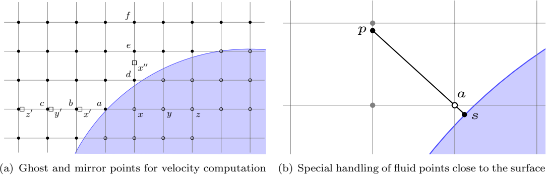
Figure 1. Immersed boundary method. (a) Ghost points ( x, y, z ; \circ ) used in the central-difference stencils of fluid points ( a-c ; \bullet ) are set by mirror points ( x', y', z' ; \square ). The mirror points are interpolated along grid lines. When ( x ; \circ ) is used to compute vertical velocity components of fluid points ( d-f ; \bullet ) the corresponding mirror point is ( x'' ; \square ). (b) For a fluid point ( a ; \circ ) very close to the cylinder surface, interpolation between a surface point ( s ; \bullet ) and the intersection between the surface normal and the first grid line at ( p ; \bullet ) is used.
