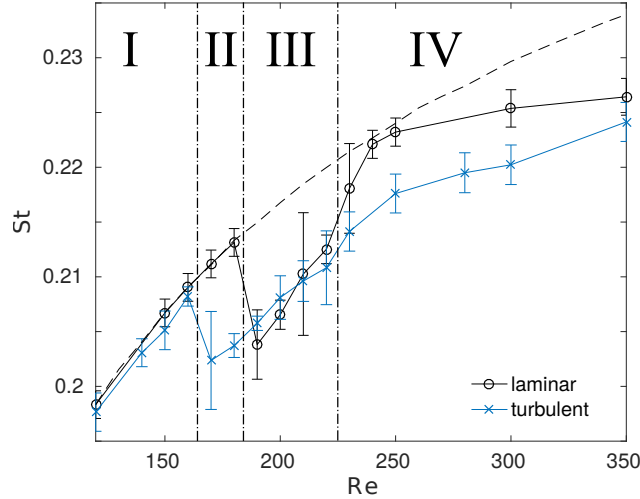
Figure 6. Comparison of St-Re relationships for flows with and without free-stream turbulence introduced upstream of the cylinder, for Reynolds numbers spanning over the transition-in-wake regime: -o- LFS; -x- TFS; - - 2D LFS.
