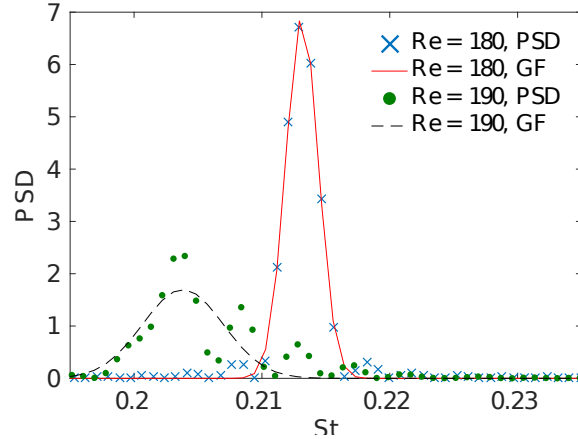
Figure 5. Power spectral density (PSD) as a function of Strouhal number with curve fitted Gaussian distribution (GF), for flow LFS flow at Re = 180 (PSD: \times , GF: —) and Re = 190 (PSD: \bullet , GF: - -).
