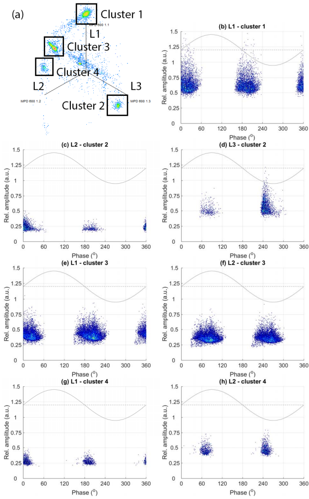
Figure 5: (a) Separation of clusters using 3PARD. PRPD patterns: (b) L1 – cluster 1, (c) L2 – cluster 2, (d) L3 – cluster 2, (e) L1 – cluster 3, (f) 2 – cluster 3, (g) L1 – cluster 4, and (h) L2 – cluster 4.
