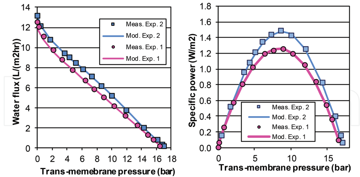
Figure 8. Water flux and specific power as functions of trans-membrane pressure for CTA membranes. Modelled values were obtained by applying a pressure dependent structure parameter.
