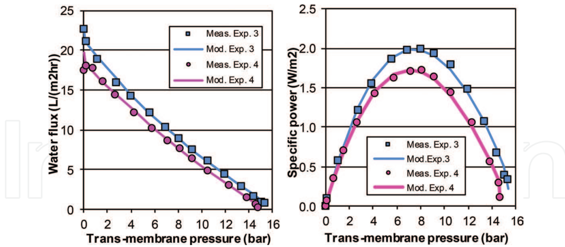
Figure 10. Water flux and specific power as functions of trans-membrane pressure for the TFC1 membrane. Modelled values were obtained by applying a pressure dependent structure parameter.
