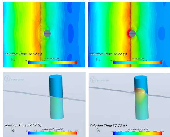
Fig. 11. Fluid visualisation of event A. (Top: free surface elevation; bottom: dynamic pressure distribution)
