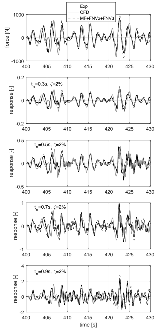
Fig. 21. Time series of the force (top) and response of the SDOF oscillator with various natural periods ( t_n ) for event B. 2% critical damping is applied in all time series shown here.
