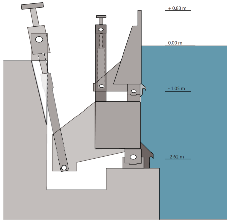
Fig. 2. MARINTEK's BM1 wavemaker [13].
