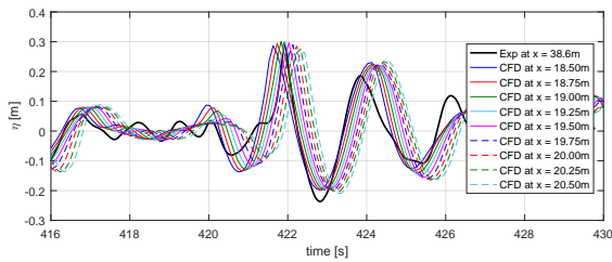
Fig. 17. Comparison of the free surface elevation at several locations against model test time series, CFD reproduction of event B vs. experiment
