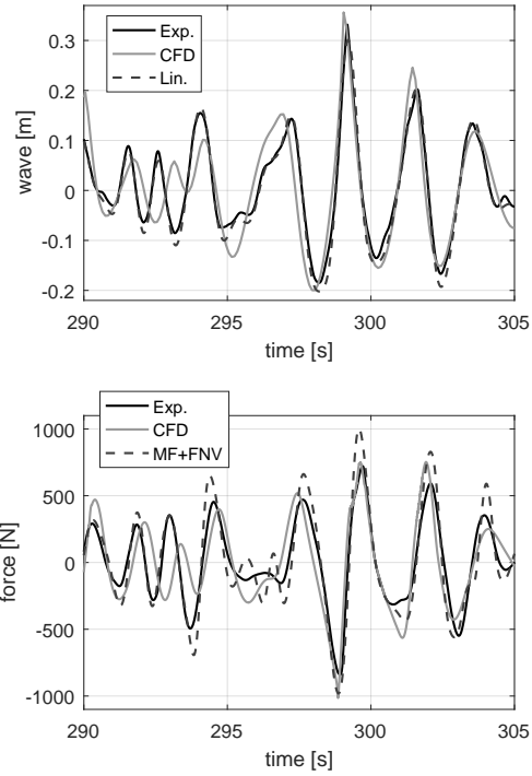
Fig. 10. Wave elevation (measured calibrated wave, CFD calibration reproduction, linearized measured wave) and corresponding force on the cylinder, event A.
