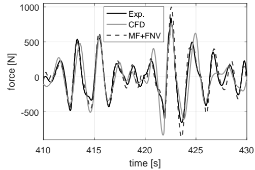
Fig. 19. Wave elevation (measured calibrated wave, CFD calibration reproduction, linearized measured wave) and corresponding force on the cylinder, event B.
