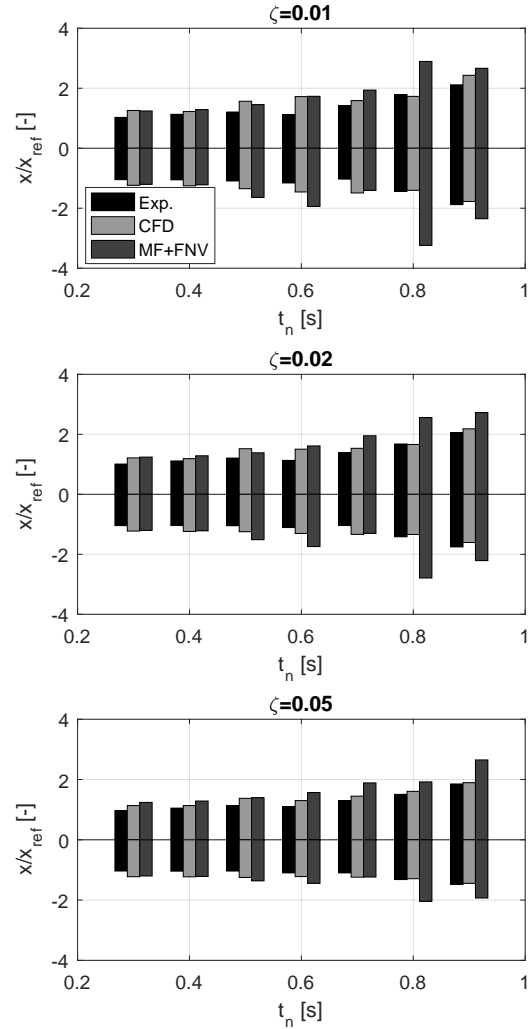
Fig. 15. Comparison of maximum positive and negative responses, event A.
