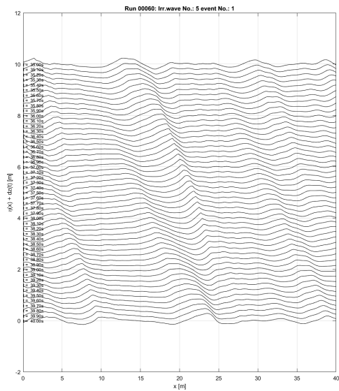
Fig. 16. Visualization of the space-time history of the CFD free surface elevation in event B.
