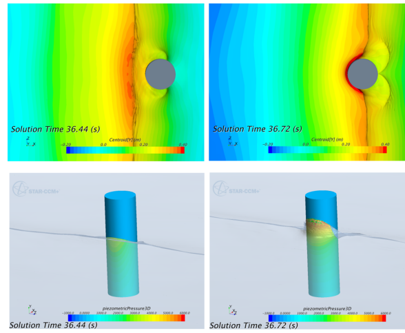
Fig. 18. Fluid visualization of event B. (Top: free surface elevation; bottom: dynamic pressure distribution)
