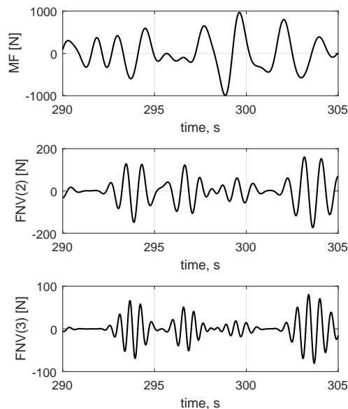
Fig. 13. Components of the hydrodynamic load according to MacCamy-Fuchs (top) and FNV second order (middle) and third order (bottom) for event A.
