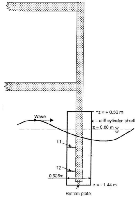
Fig. 3. Model setup [9]
