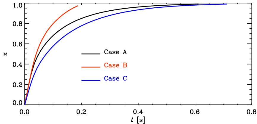
Figure 1: Carbon conversion as a function of time. (See Table 4 for descriptions of Cases A, B and C.)
