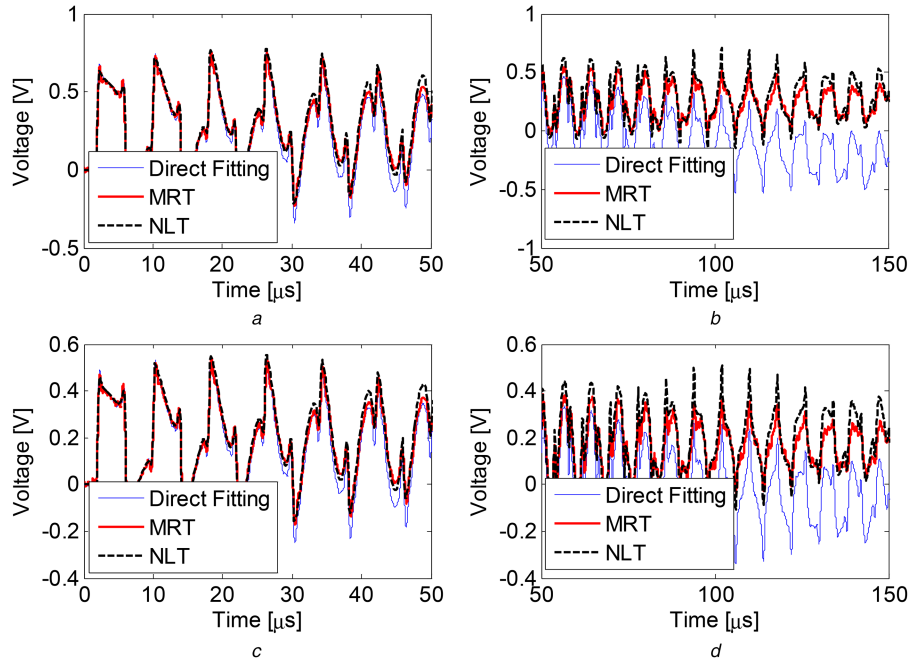
Fig. 7 Voltage considering the direct fitting, MRT and NLT approaches for the simple river crossing (a) From 0 s to 50 \mu s (node #5), (b) From 50 to 150 \mu s (node #5), (c) From 0 s to 50 \mu s (node #6), (d) From 50 to 150 \mu s (node #6)
