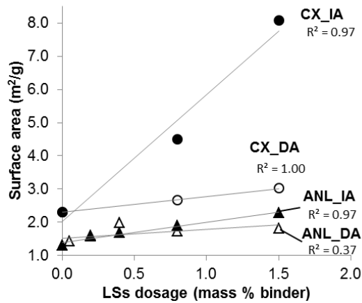
633 Figure 5 – Surface area of ANL and CX cement particles hydrated for 30 min. both for IA and DA vs. 634 the total dosage of LSs added (mass % of binder)
