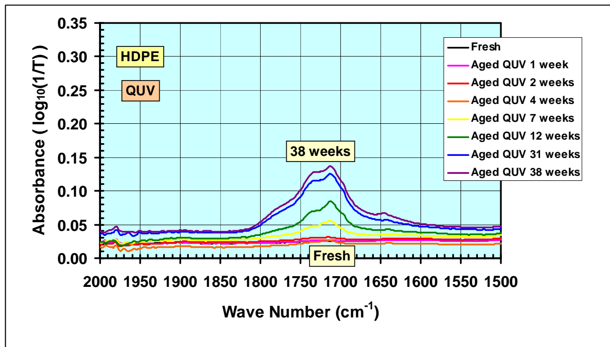
Figure 10. Absorbance (logarithmic) versus wave number between 2000-1500 cm -1 for HDPE during QUV exposure.
