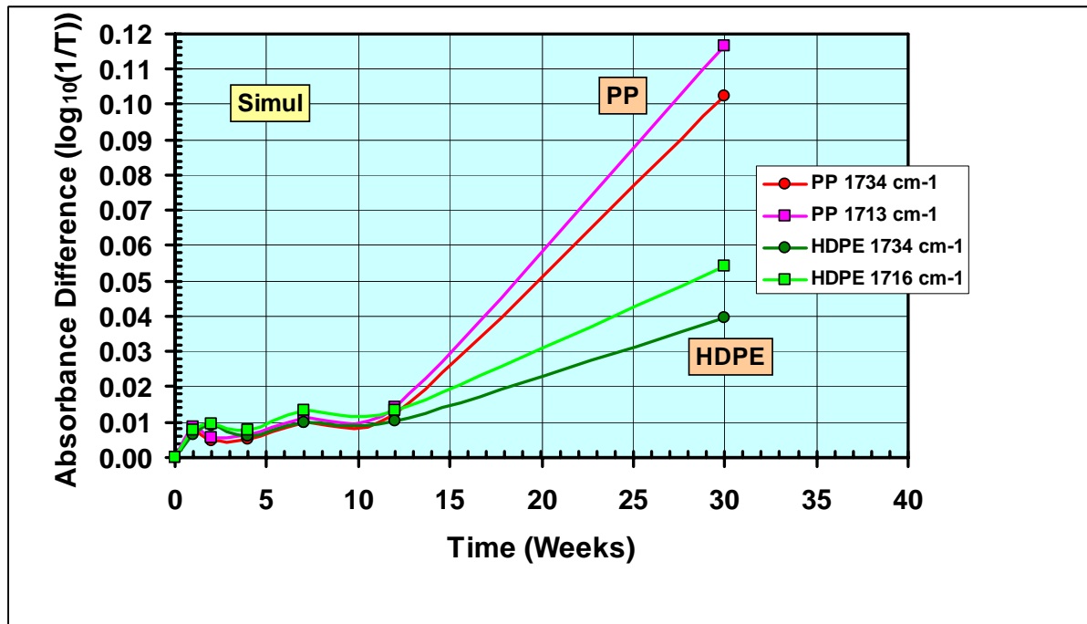
Figure 17. Absorbance difference (logarithmic) versus exposure time for PP and HDPE at wave numbers around 1732\text{ cm}^{-1} and 1713\text{ cm}^{-1} for the Simul accelerated ageing apparatus.
