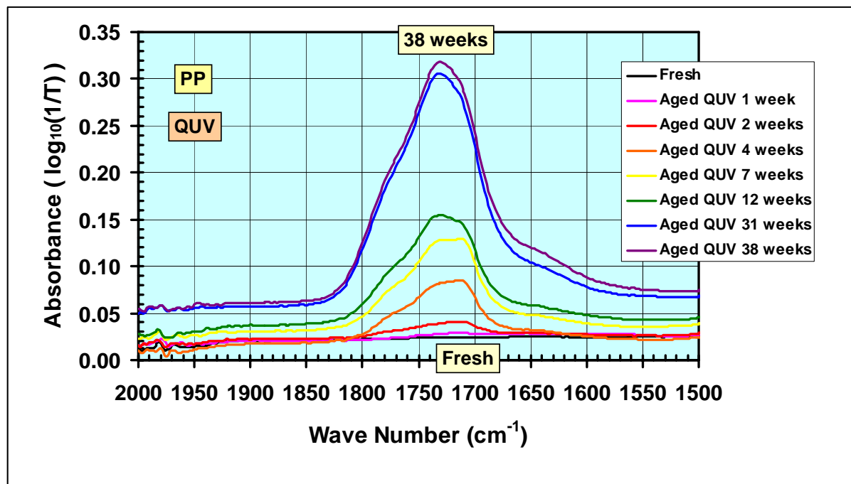
Figure 4. Absorbance (logarithmic) versus wave number between 2000-1500 cm -1 for PP during QUV exposure.
