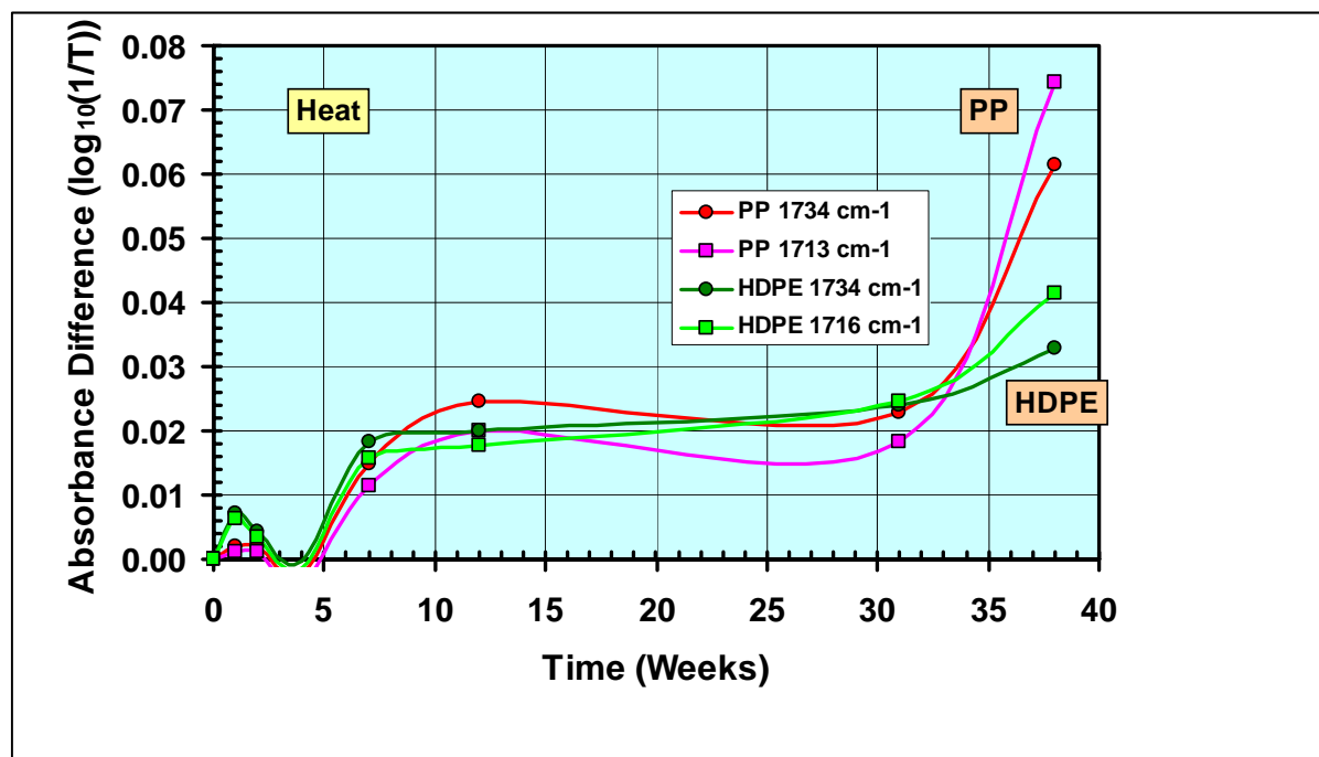
Figure 16. Absorbance difference (logarithmic) versus exposure time for PP and HDPE at wave numbers around 1734 cm -1 and 1716 cm -1 for the Heat accelerated ageing apparatus.
