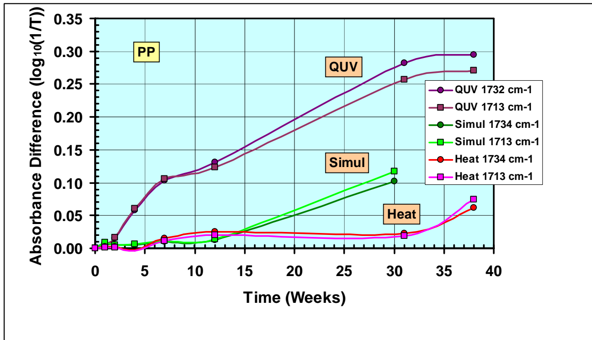
Figure 13. Absorbance difference (logarithmic) versus exposure time for PP at wave numbers around 1732 cm -1 and 1713 cm -1 for the various accelerated ageing apparatuses.
