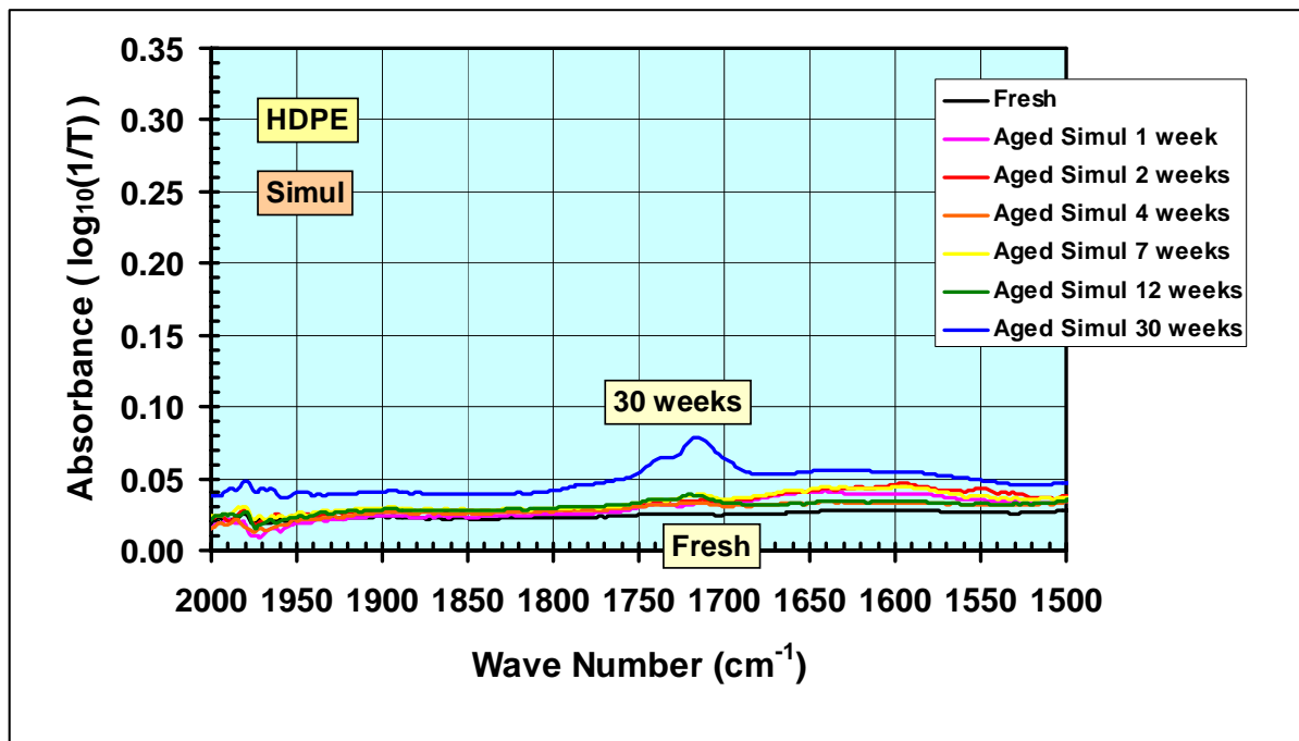
Figure 12. Absorbance (logarithmic) versus wave number between 2000-1500 cm -1 for HDPE during Simul exposure.
