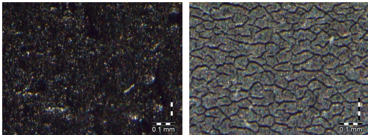
Figure 18. Microscope photos of non-aged PP (left) and QUV aged for 38 weeks PP (right), clearly depicting the crevice formation in the QUV aged PP.
