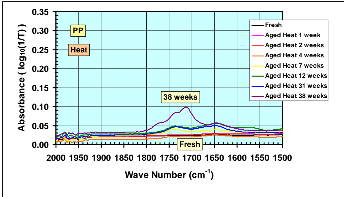
Figure 5. Absorbance (logarithmic) versus wave number between 2000-1500 \text{cm}^{-1} for PP during Heat exposure.
