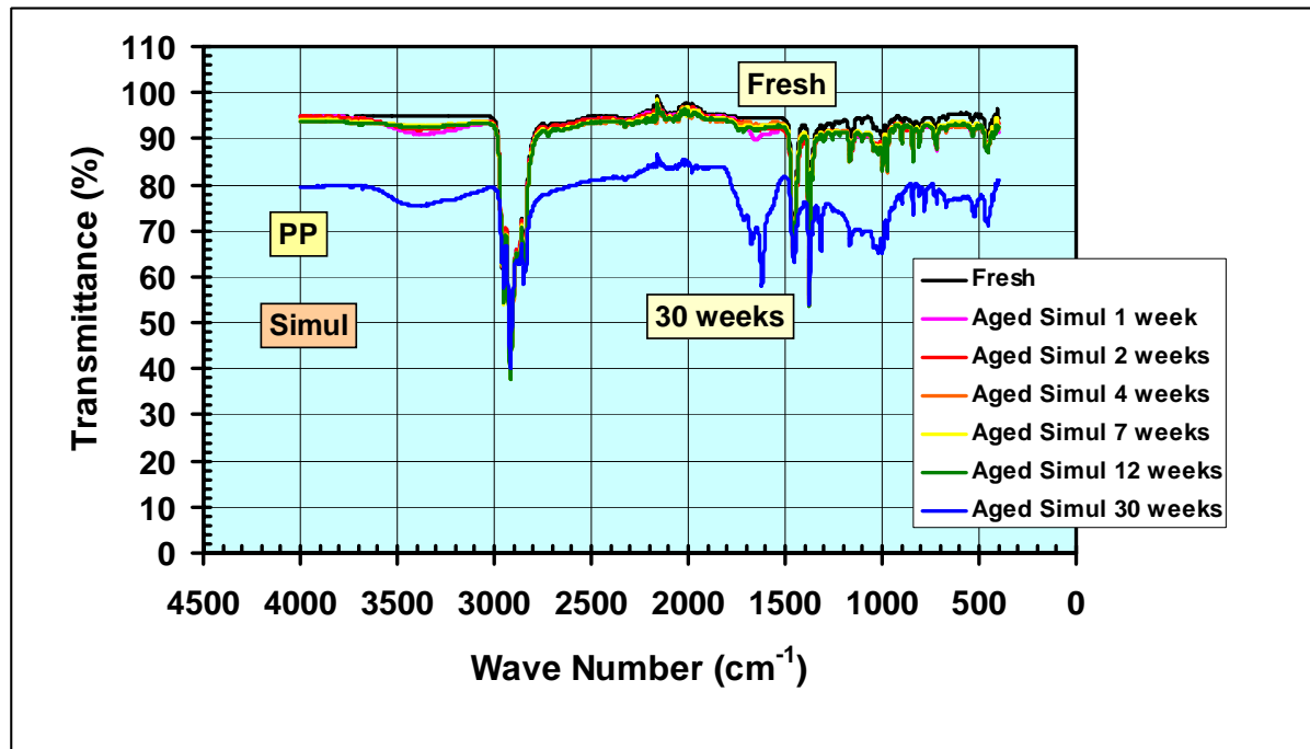
Figure 3. Transmittance versus wave number between 4000-400 cm -1 for PP during Simul exposure.
