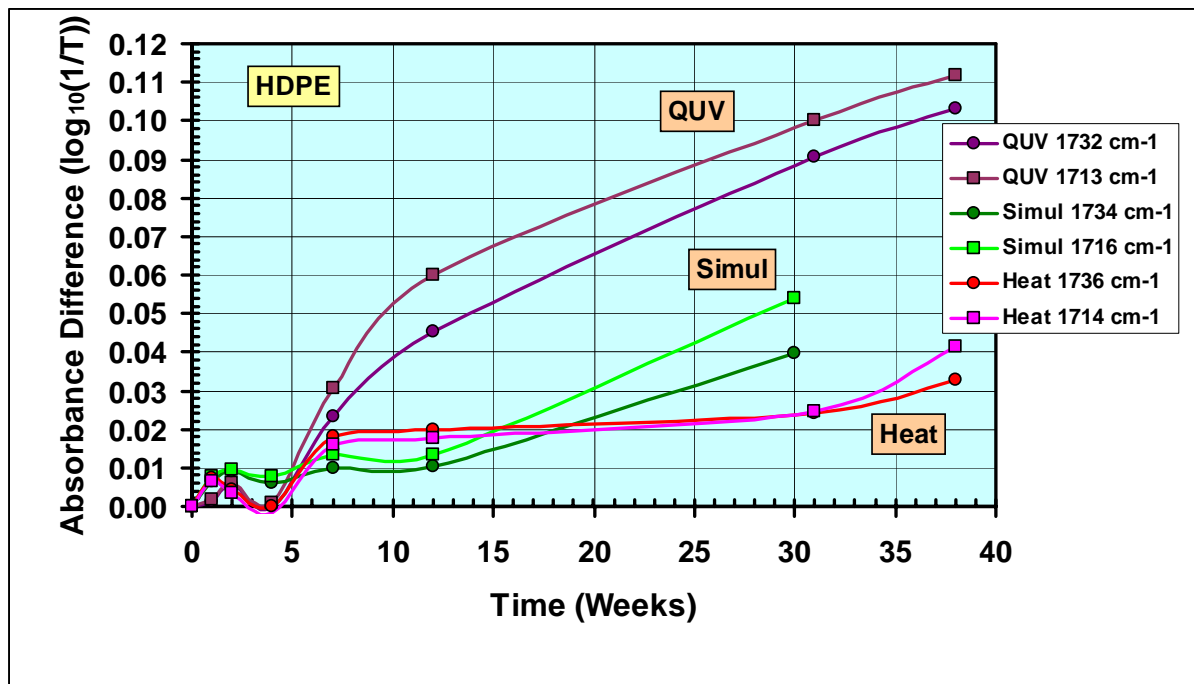
Figure 14. Absorbance difference (logarithmic) versus exposure time for HDPE at wave numbers around 1732 cm -1 and 1713 cm -1 for the various accelerated ageing apparatuses.
