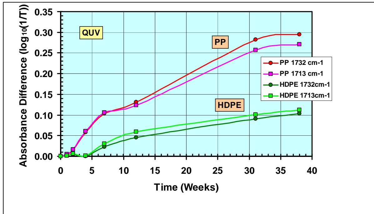
Figure 15. Absorbance difference (logarithmic) versus exposure time for PP and HDPE at wave numbers around 1732 cm -1 and 1713 cm -1 for the QUV accelerated ageing apparatus.
