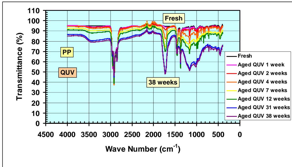
Figure 1. Transmittance versus wave number between 4000-400 \text{cm}^{-1} for PP during QUV exposure.
