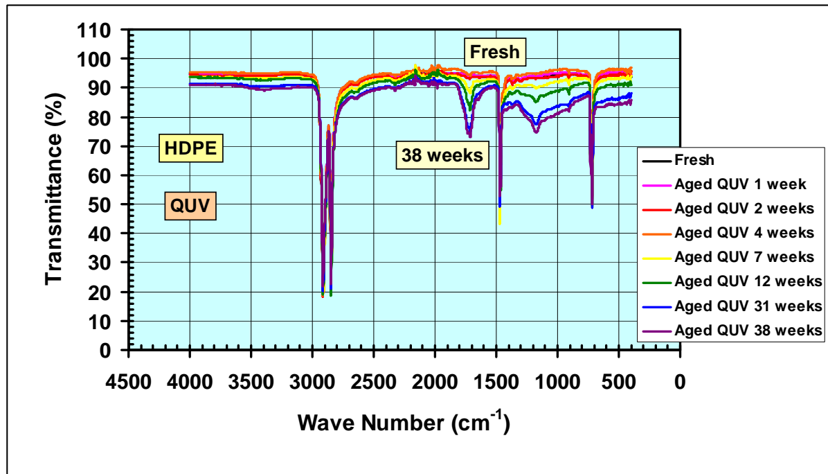
Figure 7. Transmittance versus wave number between 4000-400 \text{cm}^{-1} for HDPE during QUV exposure.
