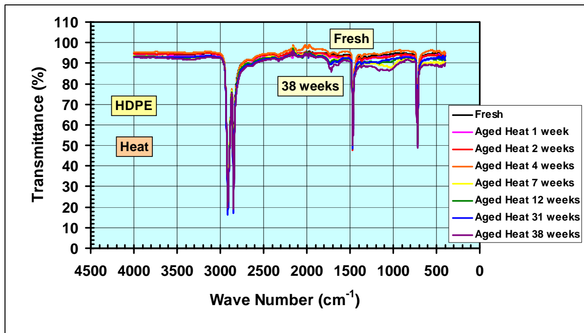
Figure 8. Transmittance versus wave number between 4000-400 \text{cm}^{-1} for HDPE during Heat exposure.
