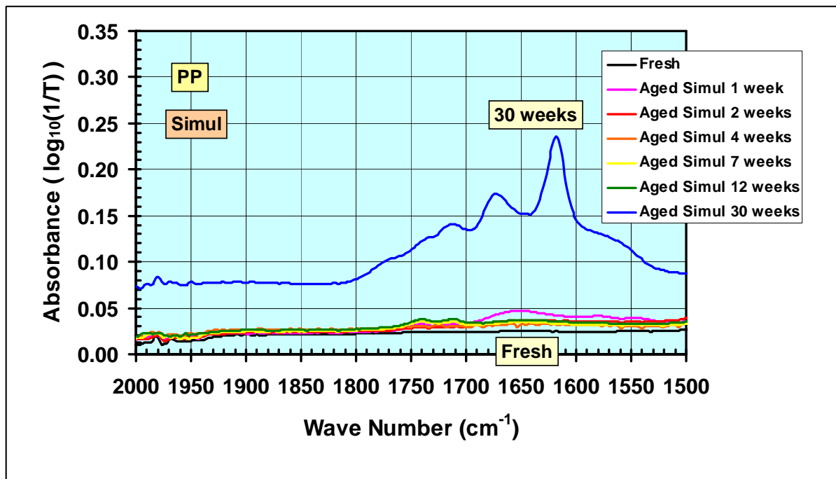
Figure 6. Absorbance (logarithmic) versus wave number between 2000-1500 \text{cm}^{-1} for PP during Simul exposure.
