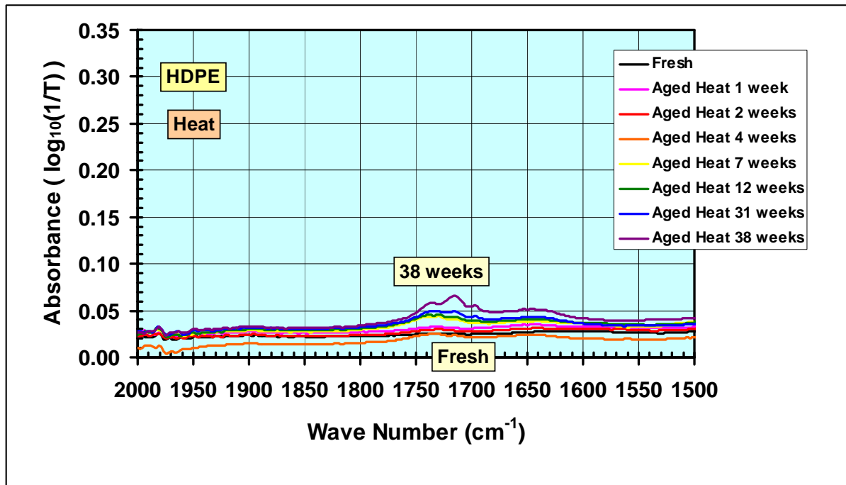
Figure 11. Absorbance (logarithmic) versus wave number between 2000-1500 cm -1 for HDPE during Heat exposure.
