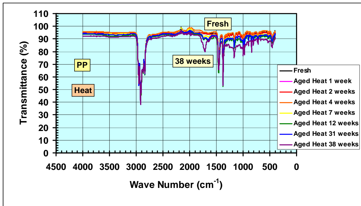
Figure 2. Transmittance versus wave number between 4000-400 \text{cm}^{-1} for PP during Heat exposure.
