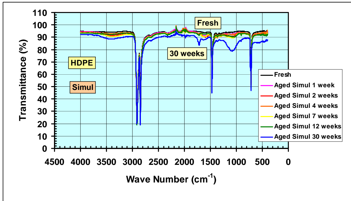
Figure 9. Transmittance versus wave number between 4000-400 cm -1 for HDPE during Simul exposure.
