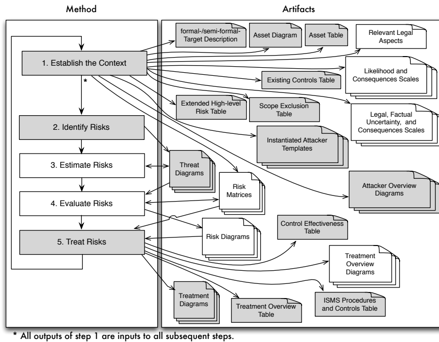
Fig. 1. The ISMS-CORAS Method
