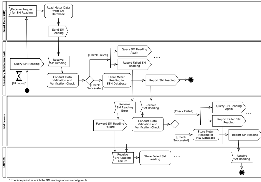
Fig. 3. Process Smart Meter Reading
