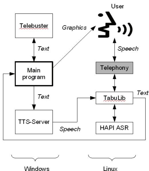
Figure 3. Marvina architecture.
