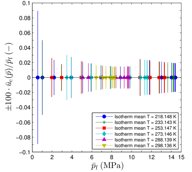
Fig. 2. Pressure standard uncertainty relative to the measured pressure for the VLE measurements performed, expressed as 100 \cdot \bar{u}_c(\bar{p})/\bar{p}_f . Measured pressure \bar{p}_f . Standard uncertainty \bar{u}_c(\bar{p}) .
