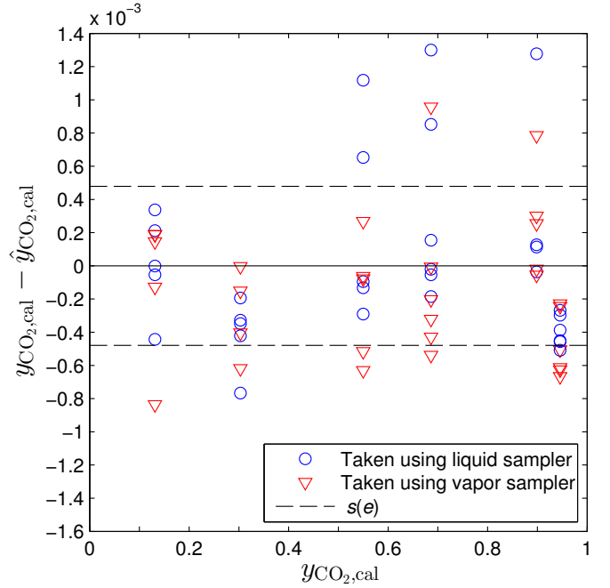
Fig. 4. Composition calibration: Error between actual compositions in Table 5 and composition model in Eq. (6), given as y_{\text{CO}_2,\text{cal}} - \hat{y}_{\text{CO}_2,\text{cal}} versus y_{\text{CO}_2,\text{cal}} . Composition analysis uncertainty u(x_{\text{CO}_2}) = u(y_{\text{CO}_2}) = s(e) from Table 6.
