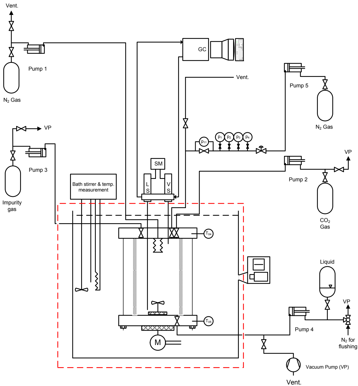
Fig. 1. Figure modified from [1]: Principal diagram of cell and ancillary apparatus. LS,VS: Liquid and vapor phase Rolsi™ samplers, respectively. SM: Rolsi™ controller. M: Gear for rotating permanent magnet below cell, which rotates stirrer inside cell. Gear connected to electric motor outside bath. T 04 : Top flange SPRT. T 05 : Bottom flange SPRT.
