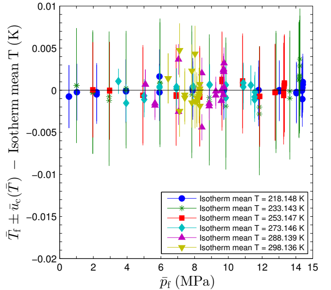
Fig. 3. Temperature deviations for each VLE measurement from isotherm mean temperature, and temperature standard uncertainty, expressed together as \bar{T}_f \pm \bar{u}_c(\bar{T}) - \text{isotherm mean temperature} , versus VLE experiment pressure \bar{p}_f . VLE experiment mean temperature \bar{T}_f . Temperature standard uncertainty \bar{u}_c(\bar{T}) .
